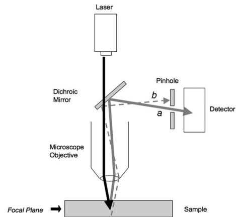
Figure 1. All confocal microscopes are based on basic property of the compound microscope: the light paths from any point in the focal plane pass through the objective and converge at a second point in the image plane of the objective. The image plane is what the oculars of the microscope project onto the eye. These two points, one in the focal plane of the object, and the other some distance behind the objective, are conjugate foci of the objective, or confocal points. In the laser-scanning confocal microscope, a beam of monochromatic laser light passes through a dichroic mirror and induces fluorescence in a discrete volume of a sample. The light emitted by the sample back through the objective is reflected towards a detector by the dichroic mirror. A plate with an adjustable diameter pinhole is placed in the light path before the detector in the image plain of the objective, so that a point in the focal plane of the sample and the pinhole are confocal. Light emitted from the focal plane will pass through the pinhole (path a ), whereas out-of-focus light emitted from outside the focal plane will be blocked (path b ).
